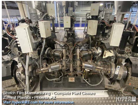
Colines ESTR Perform EX 120, 80 & 65 mm Extruders
